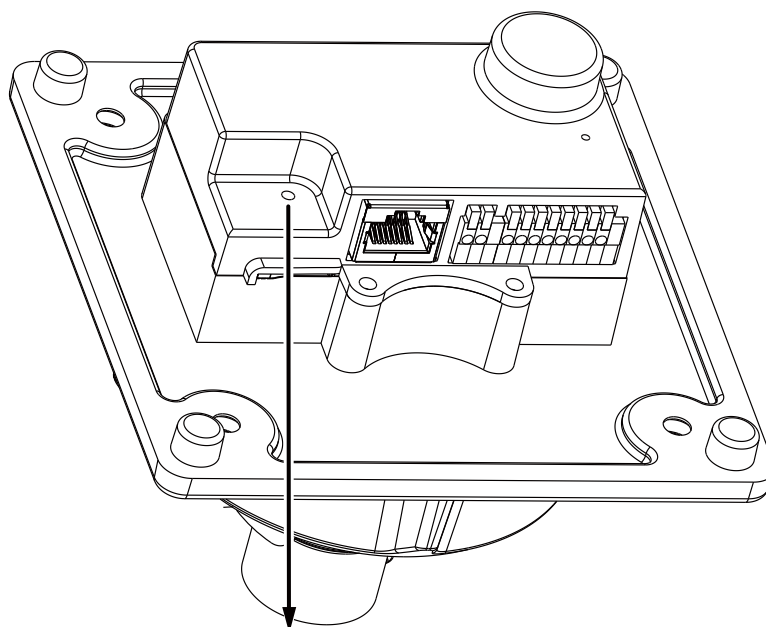
Reset Button
