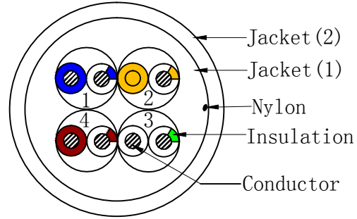
CROSS-SECTION
